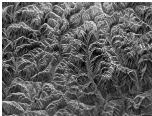
Spaceborne radar image of mountainous region in southeast Tibet
