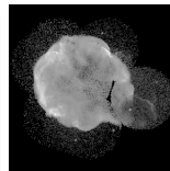
Cygnus loop
